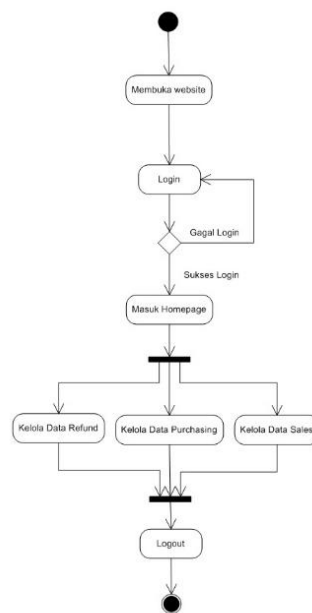
Gambar 1. Activity Diagram Admin
